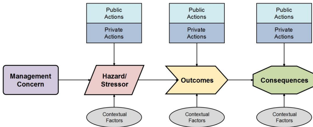
Figure 1: Building blocks of a VCAPS diagram.
