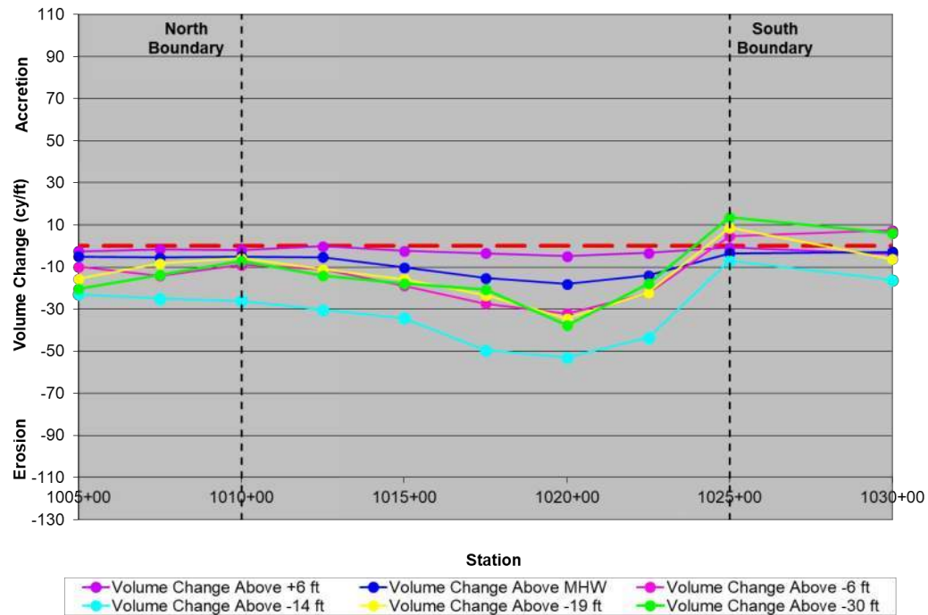
Figure 5-23. Nags Head – Reach 4 Unit Volume Change (June 2023 – June 2024)
