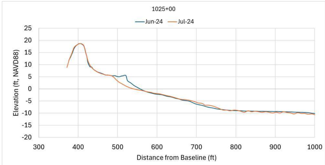
Figure 9. Transect STA 1025+00 Observed Change, June to July 2024.
