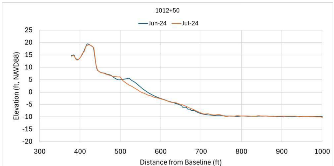
Figure 4. Transect STA 1012+50 Observed Change, June to July 2024.
