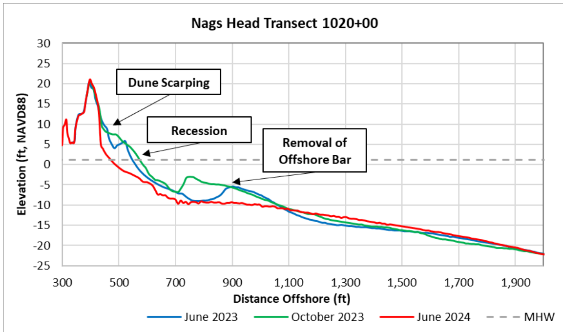
Figure 5-24. Example Reach 4 Profile, Station 1020+00 (McCall Court)
