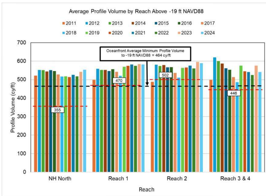
Figure 6-4. Master Plan Nourishment Trigger Volume Comparison
