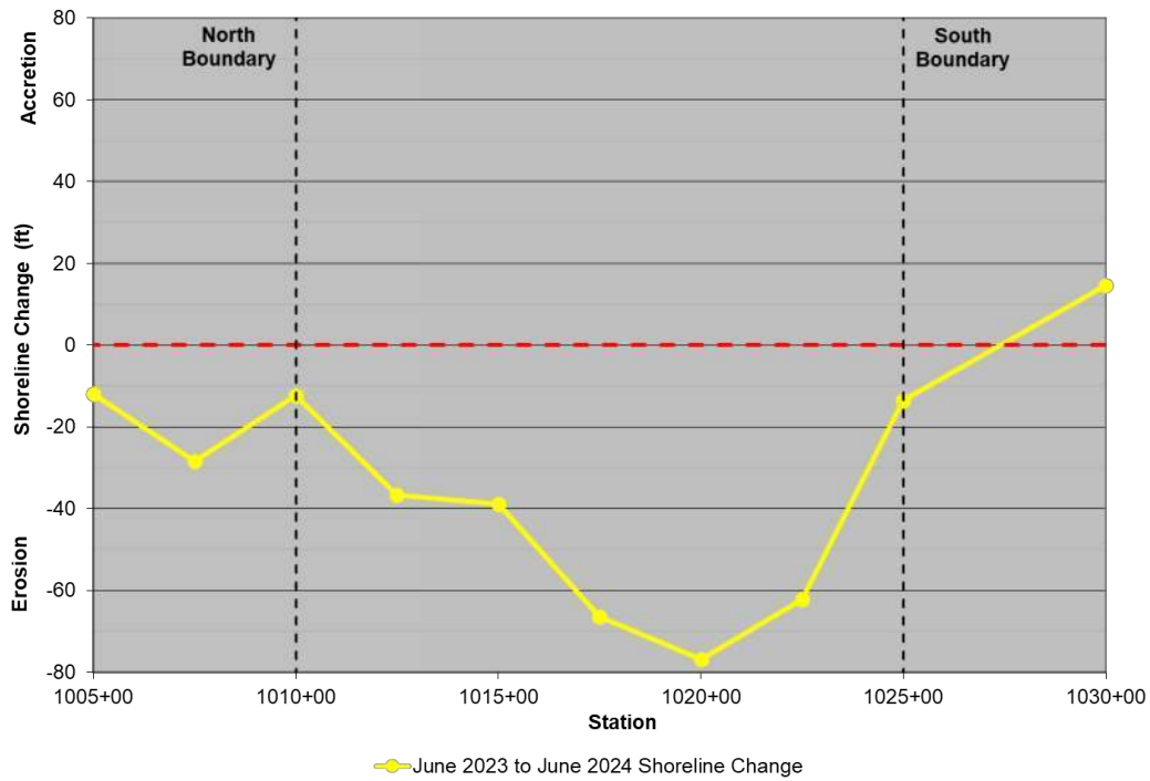
Figure 5-22. Nags Head – Reach 4 Shoreline Change (June 2023 – June 2024)
