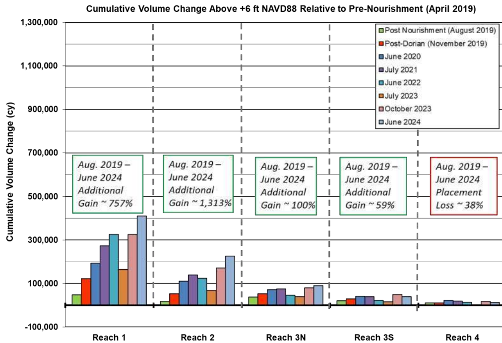
Figure 5-35. Cumulative Volume Change Above +6 ft NAVD88 Relative to Pre-Nourishment
