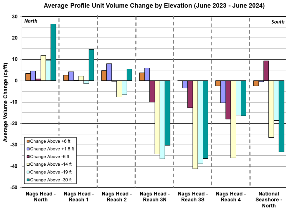
Figure 5-31. Average Unit Volume Change Within Each Reach (June 2023 – June-July 2024)
