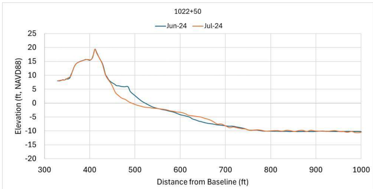
Figure 8. Transect STA 1022+50 Observed Change, June to July 2024.
