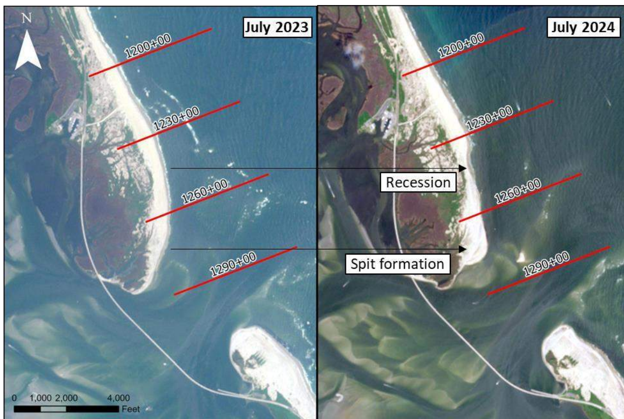
Figure 5-29. Oregon Inlet Change (07/01/2023 USGS Sentinel Imagery; 07/20/2024 USGS-Sentinel Imagery)
