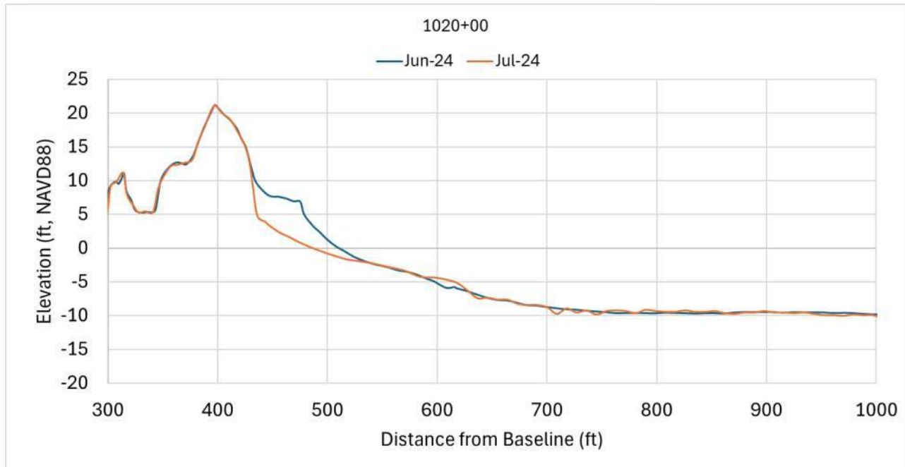
Figure 7. Transect STA 1020+00 Observed Change, June to July 2024.
