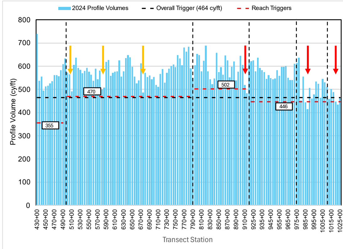
Figure 6-5. 2024 Beach Profile Volumes and Master Plan Trigger Volume Comparison. Red arrows indicate locations that are below the trigger volumes and yellow areas indicate areas that are close to the trigger volumes.
