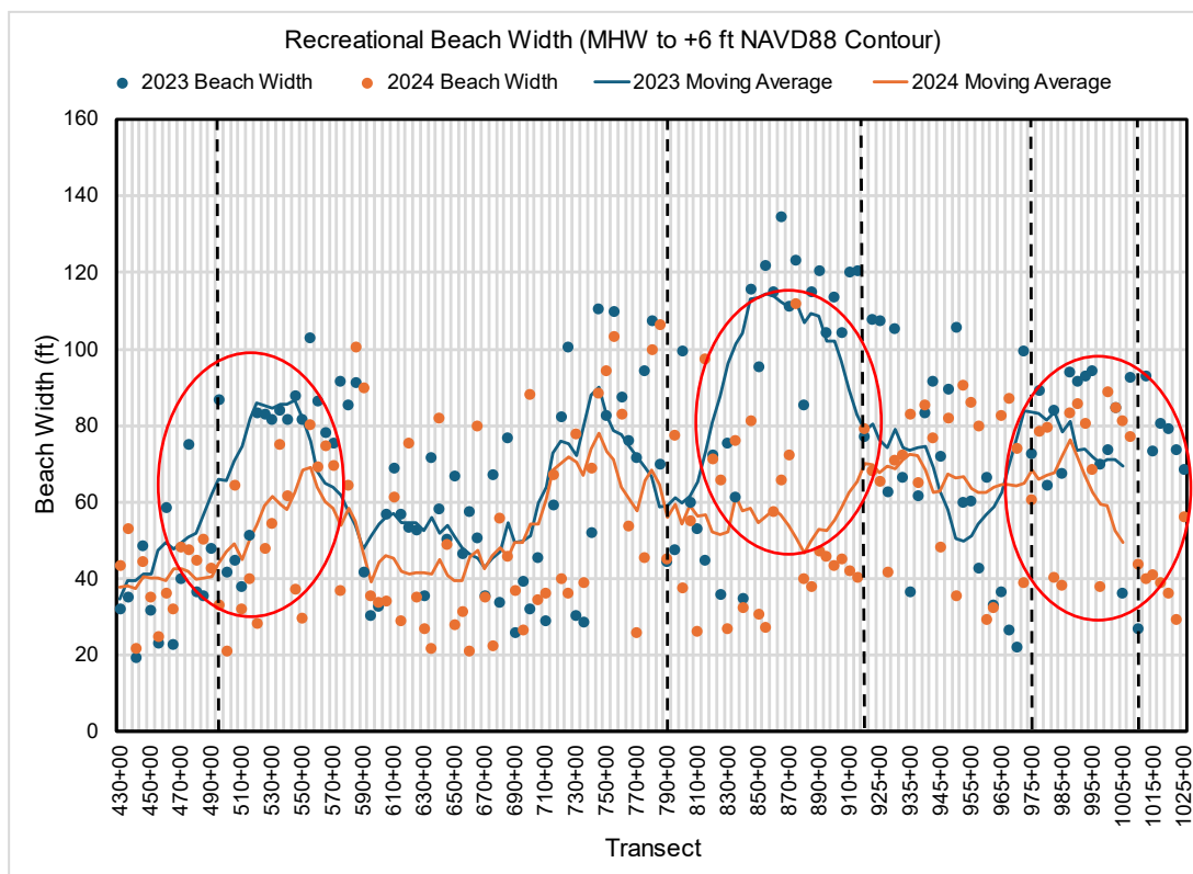
Figure 5-40. Recreational Beach Width Comparison, 2023 to 2024
