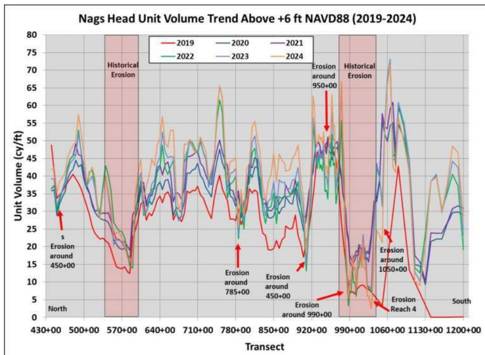
Figure 5-44. Unit Dune Volume by Year (Moving Average Trend Above +6 ft NAVD88)
