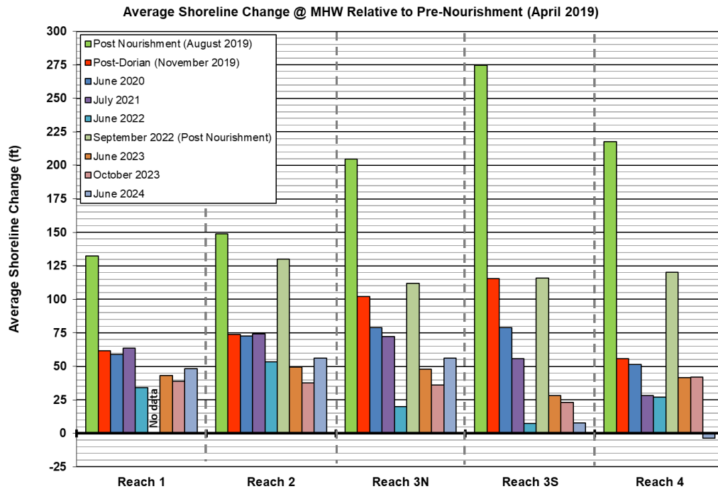
Figure 5-33. Nourished Oceanfront Average Shoreline Change Relative to Pre-Nourishment Conditions
