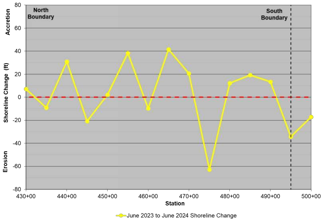
Figure 5-5. Nags Head – North Shoreline Change (June 2023 – June 2024)
