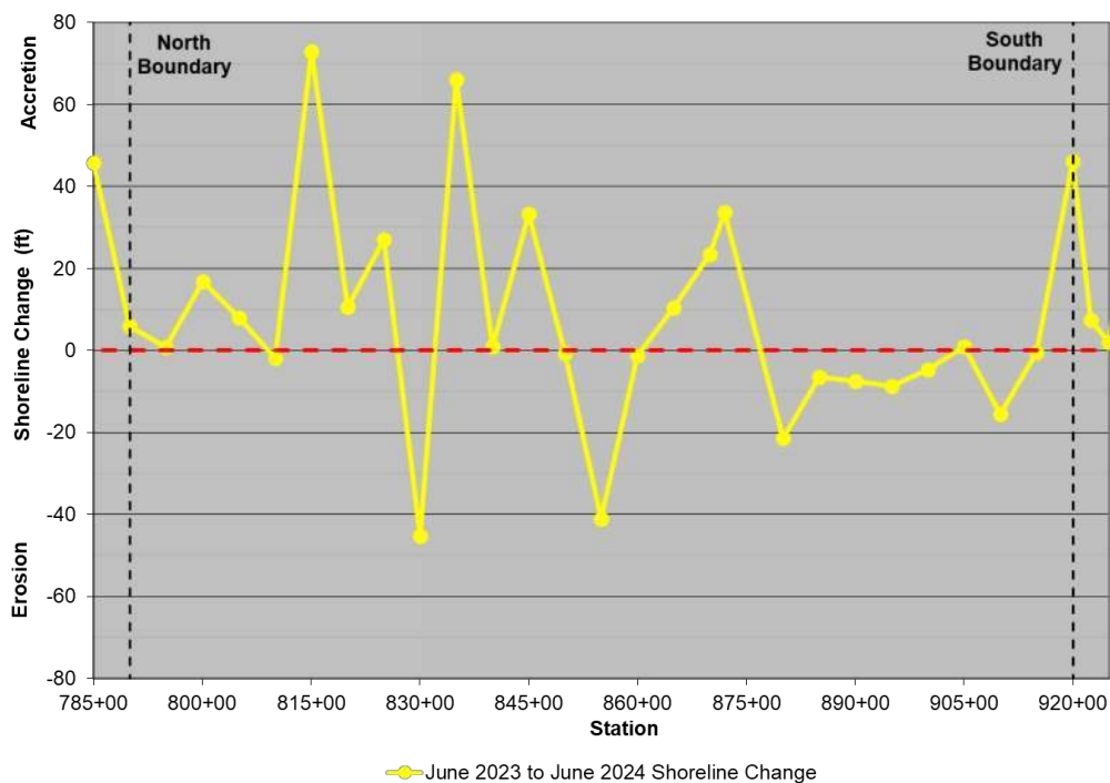
Figure 5-12. Nags Head – Reach 2 Shoreline Change (June 2023 – June 2024)
