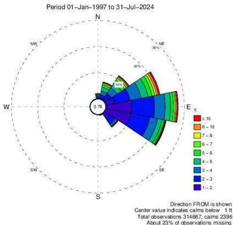
Figure 5-4. Station 44056 Significant Wave Height Rose from January 1997 – July 2024
