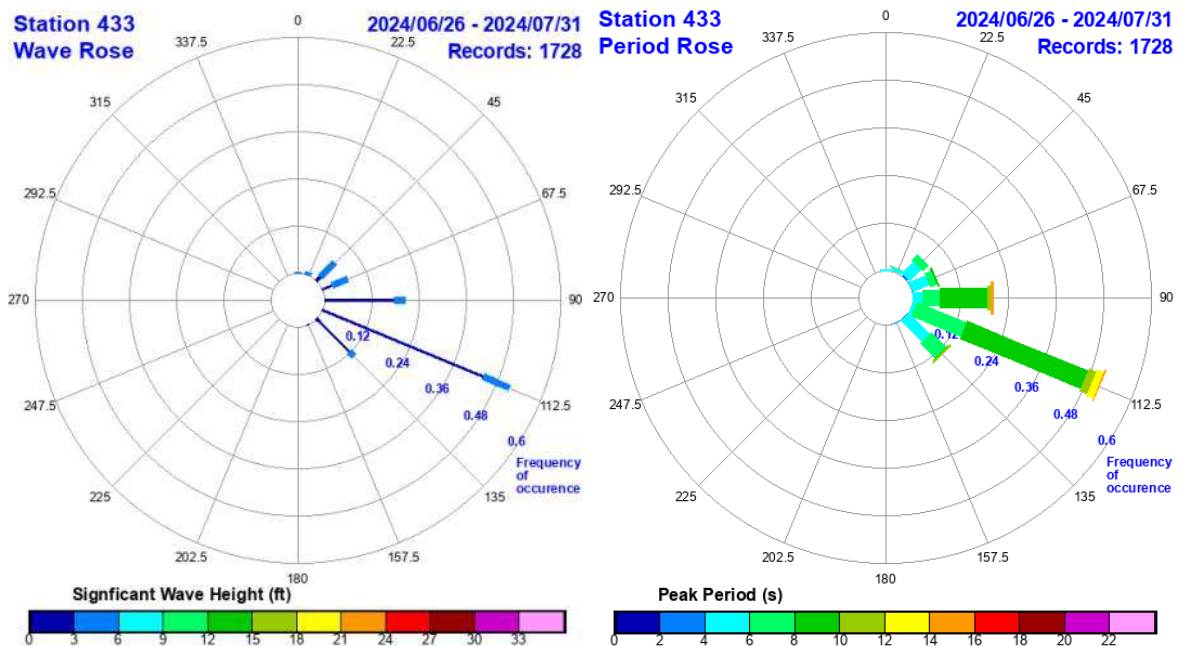
Figure 10. Wave Height (left) and Wave Period (right) Roses for June 26, 2024 to July 31, 2024, at Station 433 (Duck -51ft waverider buoy).
