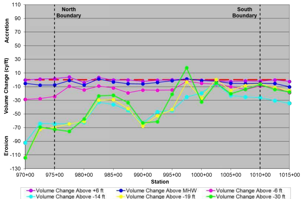
Figure 5-19. Nags Head – Reach 3 – S Unit Volume Change (June 2023 – June 2024)
