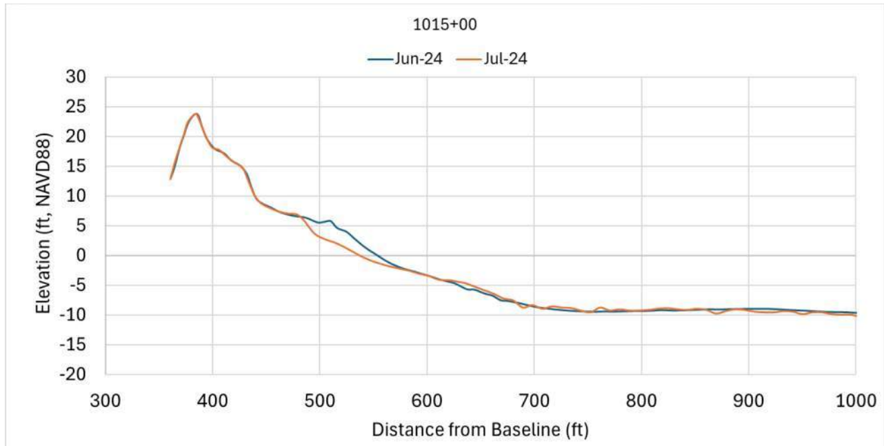
Figure 5. Transect STA 1015+00 Observed Change, June to July 2024.
