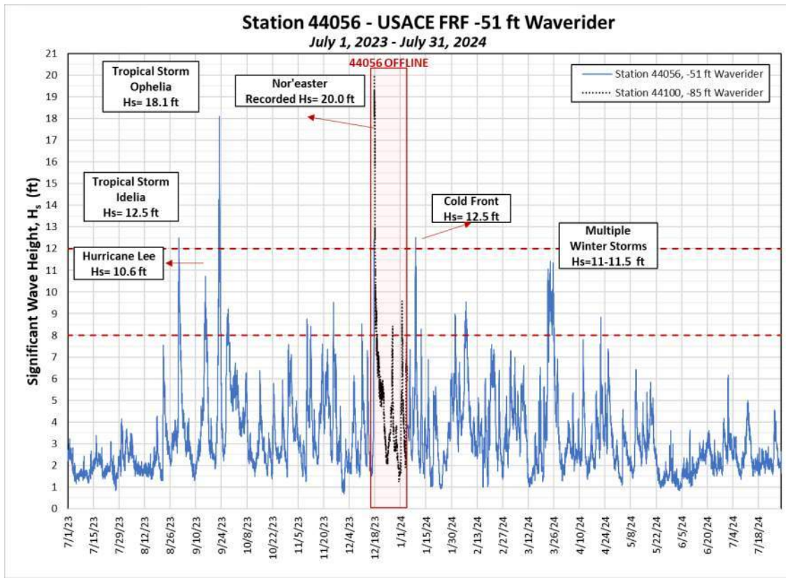
Figure 5-2. USACE FRF Station 44056 Wave Height
