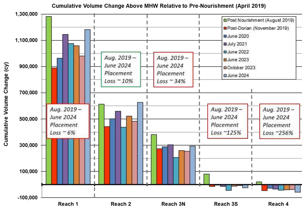
Figure 5-36. Cumulative Volume Change Above MHW Relative to Pre-Nourishment
