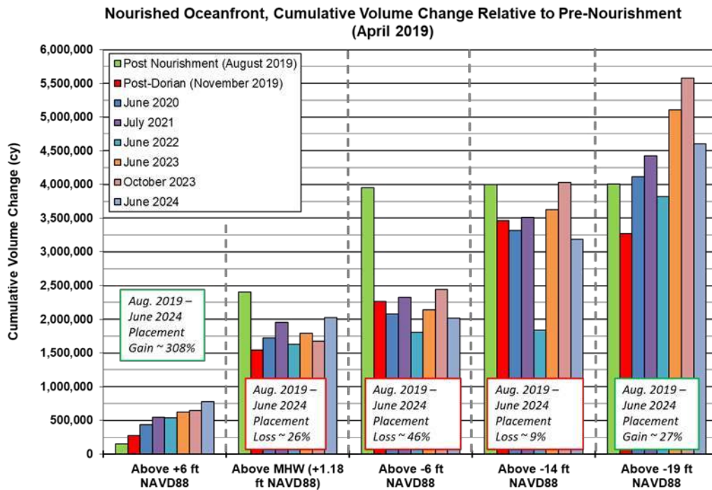
Figure 6-2. Nourished Oceanfront Cumulative Volume Change Relative to Pre-Nourishment
