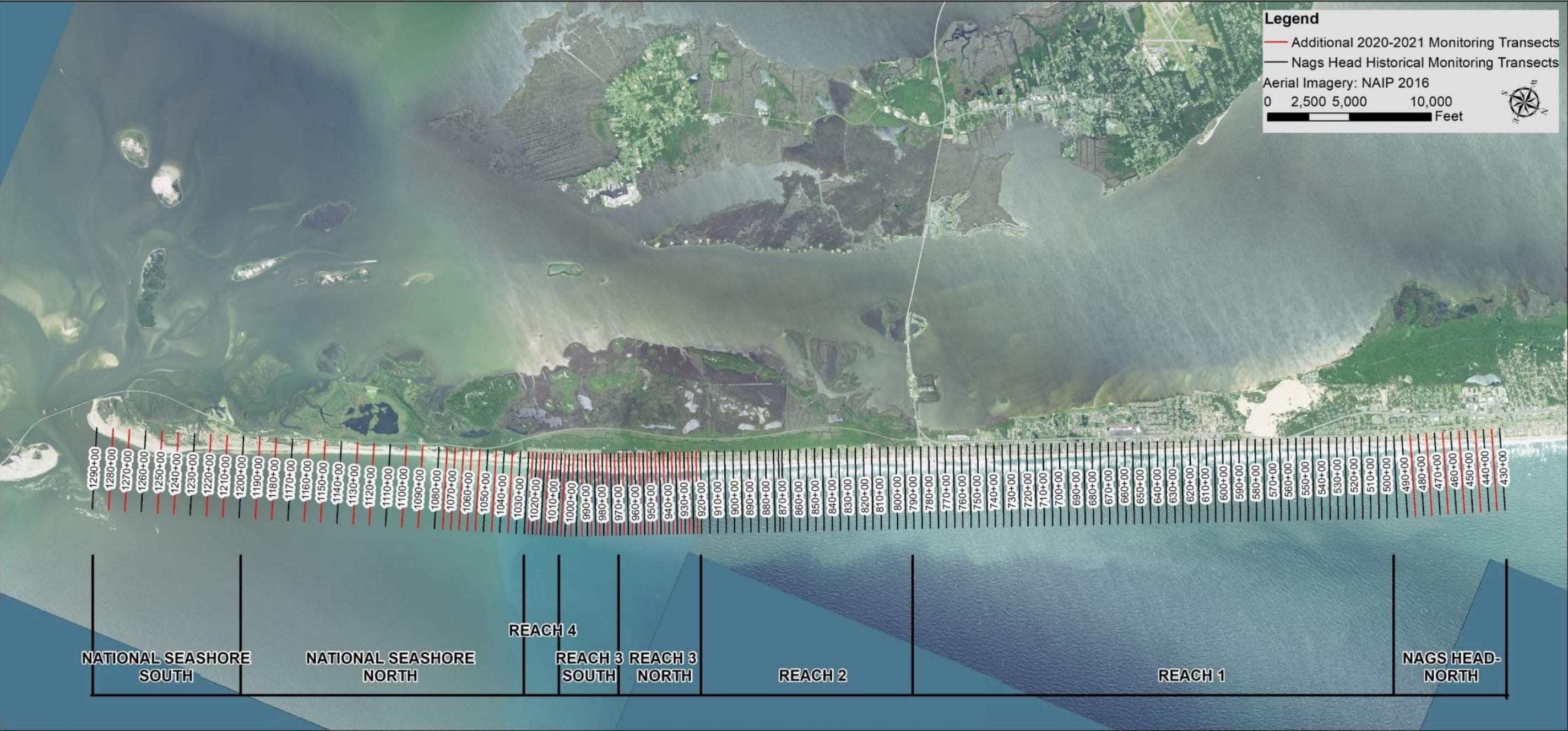
Figure 3-1. Nags Head Annual Monitoring Profile Line Locations
