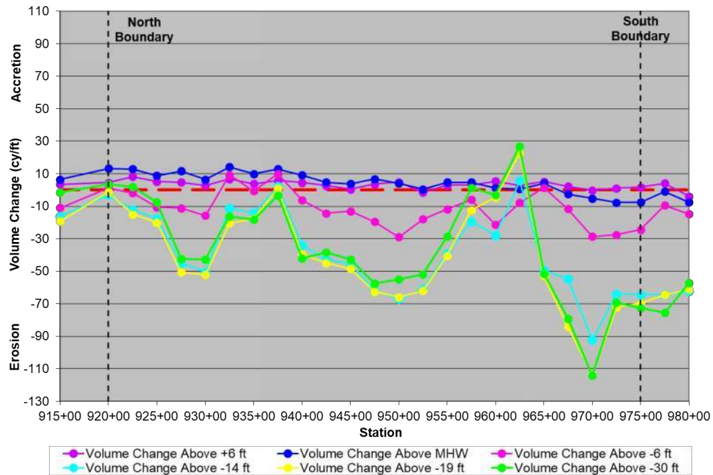
Figure 5-16. Nags Head – Reach 3 - N Unit Volume Change (June 2023 – June 2024)
