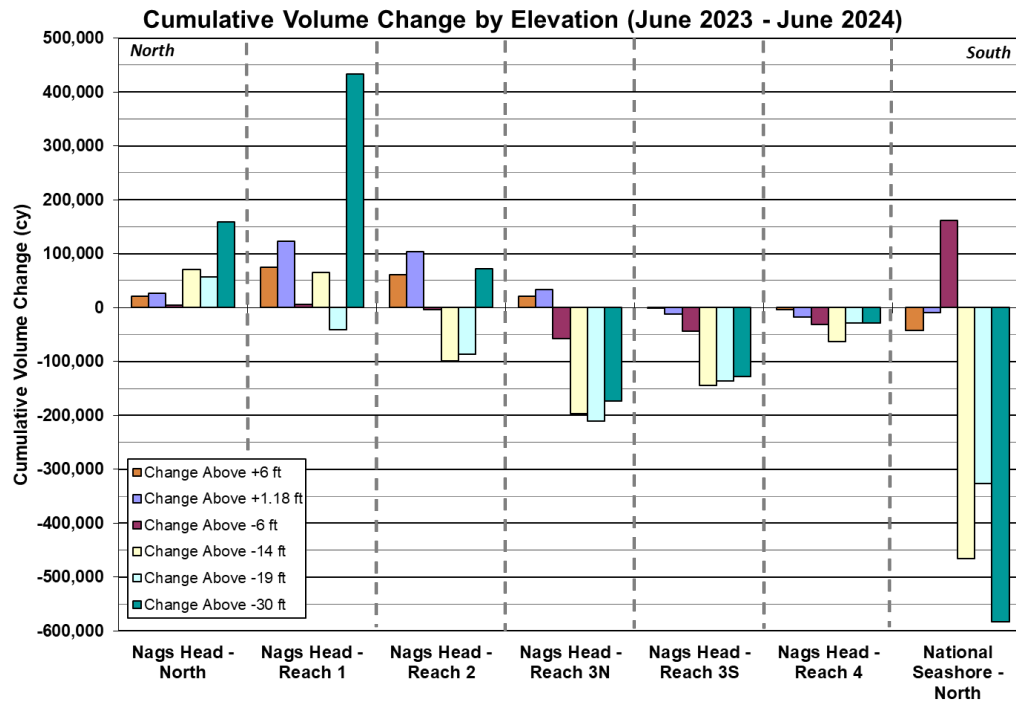
Figure 5-32. Cumulative Volume Change Within Each Reach (June 2023 – June-July 2024)
