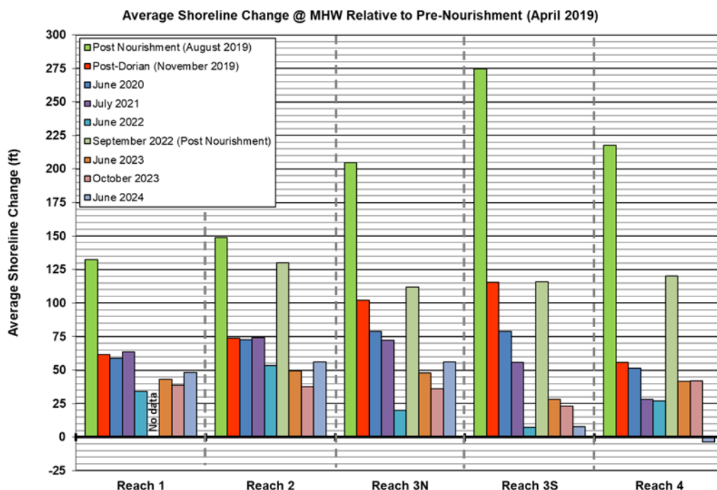
Figure ES-1. Nourished Oceanfront Average Shoreline Change Relative to Pre-Nourishment Conditions
