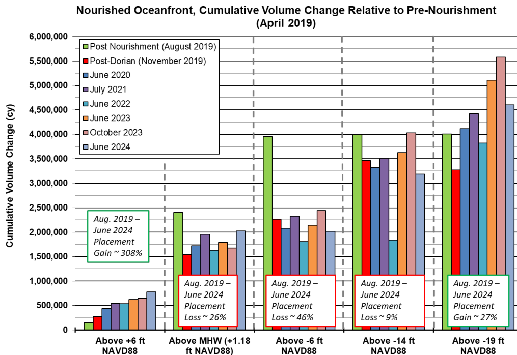
Figure 5-34. Nourished Oceanfront Cumulative Volume Change Relative to Pre-Nourishment
