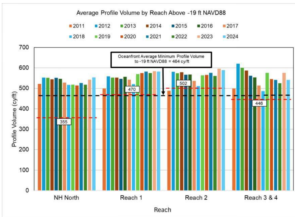
Figure ES-4. Master Plan Nourishment Trigger Volume Comparison
