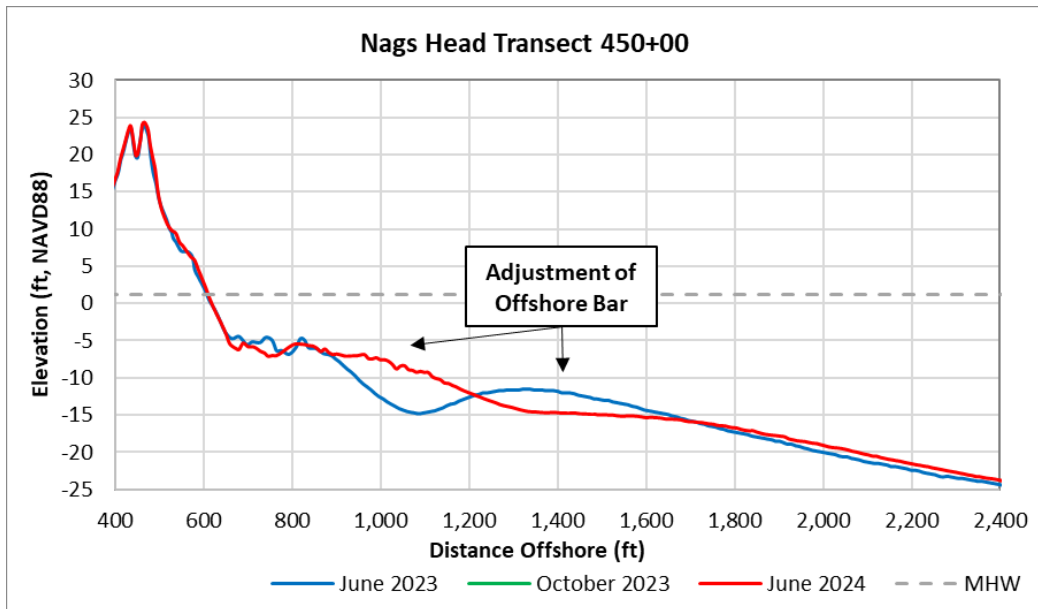
Figure 5-7. Example Nags Head – North Profile, Station 450+00 (E. Albatross St.)
