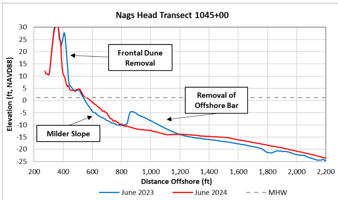
Figure 5-27. Example National Seashore - North Profile, Station 1045+00
