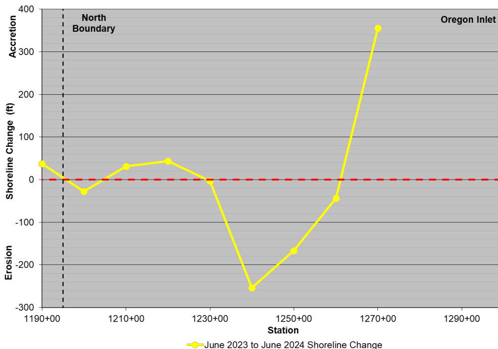
Figure 5-28. National Seashore - South Shoreline Change (2023 – 2024)
