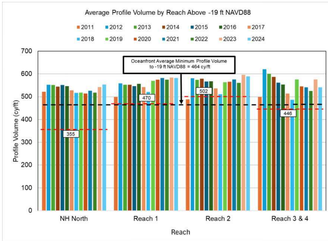
Figure 5-38. Master Plan Nourishment Trigger Volume Comparison
