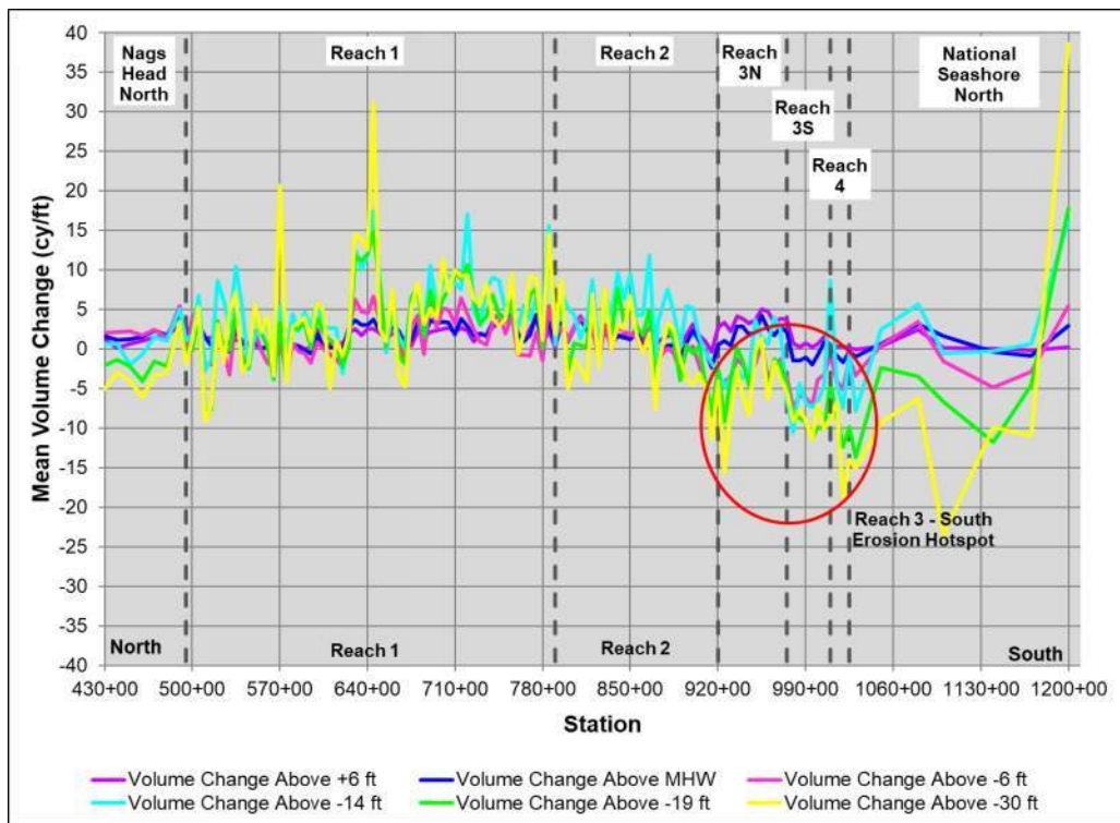
Figure 5-41. Mean Volume Change per year (2011 – 2024) (With Nourishment)
