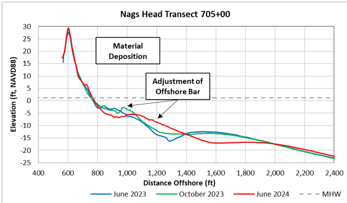
Figure 5-11. Example Reach 1 Profile, Station 705+00 (E Sea Spray Ct.)
