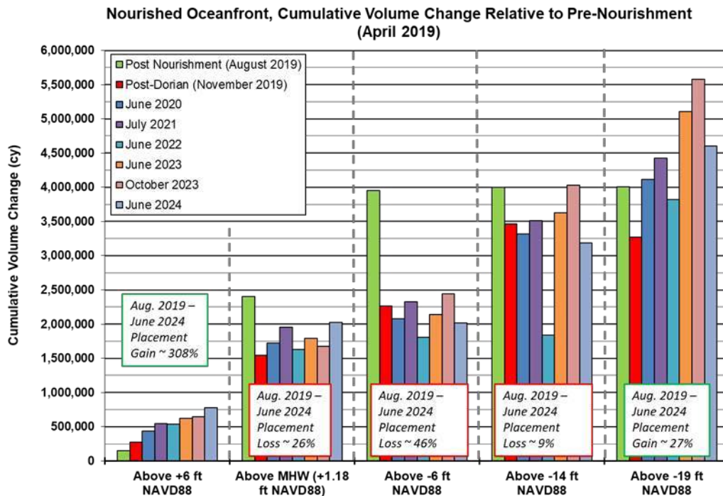
Figure ES-2. Nourished Oceanfront Cumulative Volume Change Relative to Pre-Nourishment
