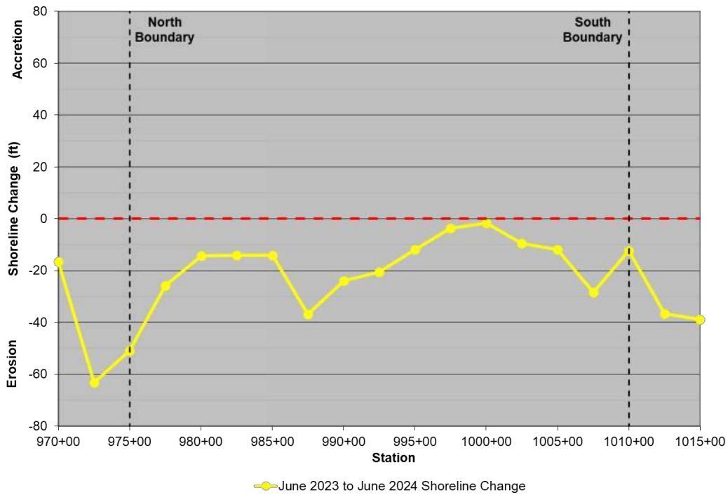
Figure 5-18. Nags Head – Reach 3 – S Shoreline Change (June 2023 – June 2024)
