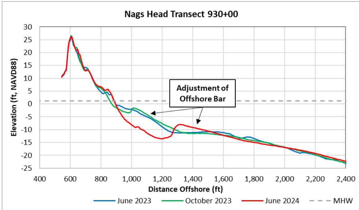
Figure 5-17. Example Reach 3 - North Profile, Station 930+00 (E Jacobs St.)
