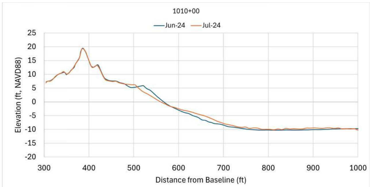
Figure 3. Transect STA 1010+00 Observed Change, June to July 2024.
