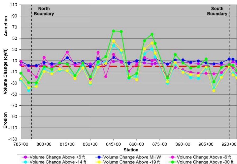
Figure 5-13. Nags Head – Reach 2 Unit Volume Change (June 2023 – June 2024)
