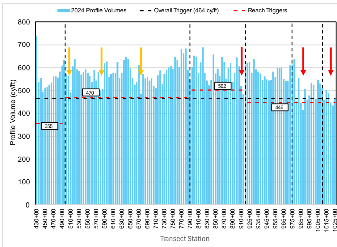
Figure 5-39. 2024 Beach Profile Volumes and Master Plan Trigger Volume Comparison. Red arrows indicate locations that are below the trigger volumes and yellow areas indicate areas that are close to the trigger volumes.
