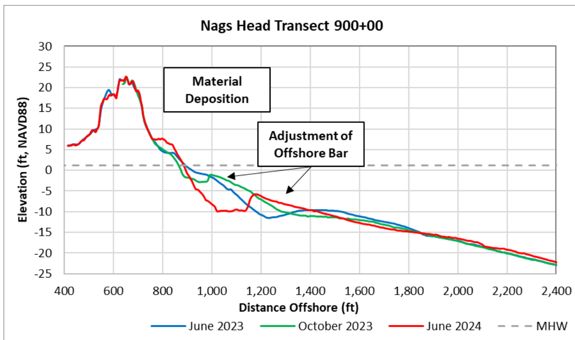
Figure 5-14. Example Reach 2 Profile, Station 900+00 (E Jay St.)
