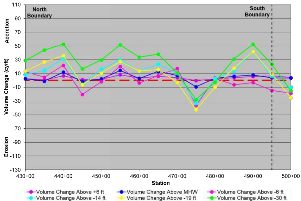
Figure 5-6. Nags Head – North Unit Volume Change (June 2023 – June 2024)
