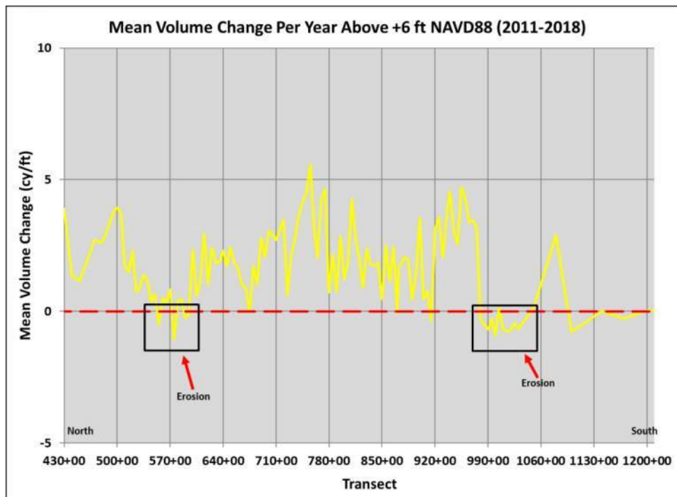
Figure 5-43. Unit Dune Volume Change from 2011 to 2018 (Moving Average Trend Above +6 ft NAVD88)
