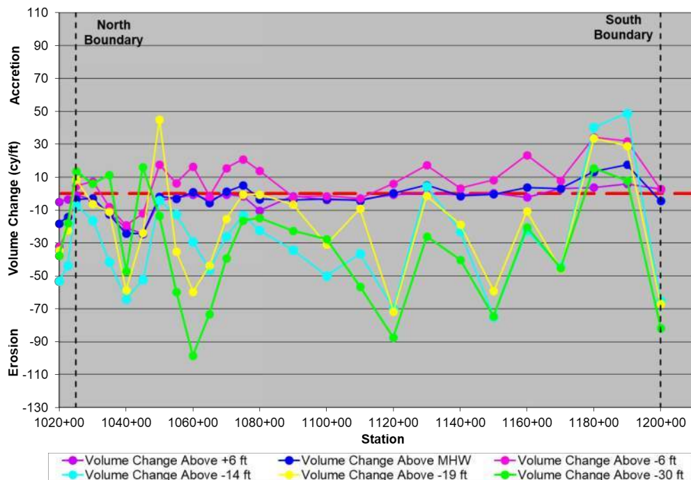
Figure 5-26. National Seashore - North Unit Volume Change (June 2023 – June 2024)
