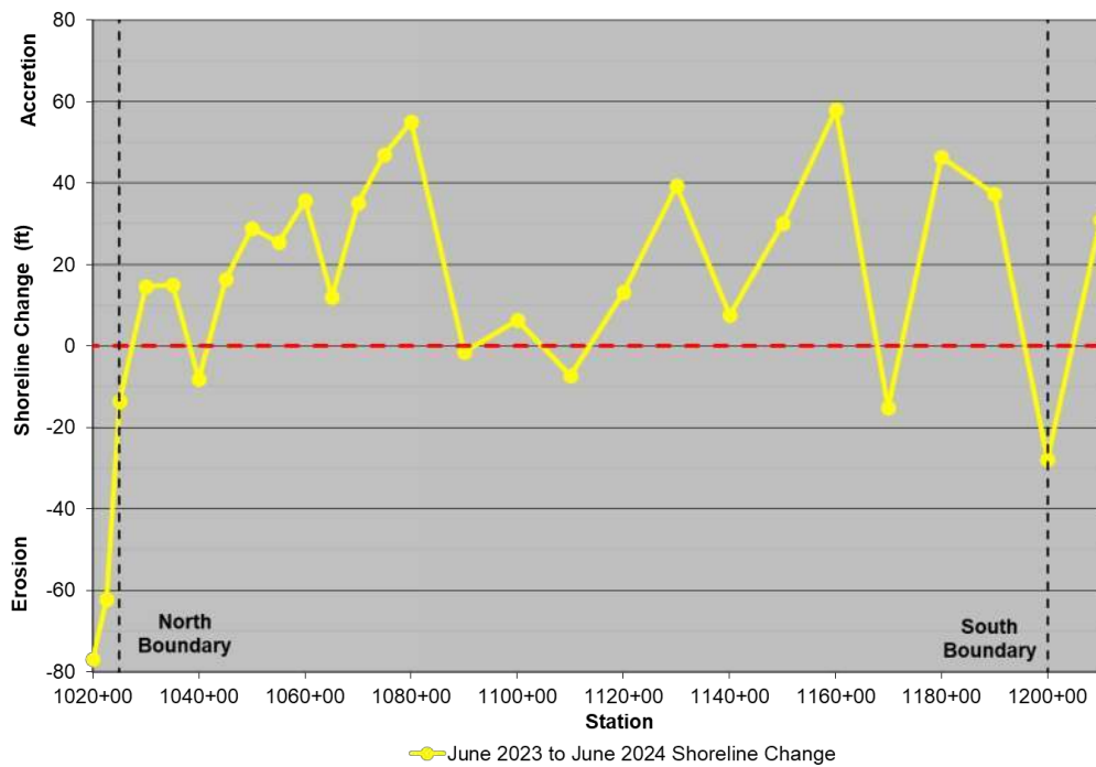
Figure 5-25. National Seashore - North Shoreline Change (June 2023 – June 2024)
