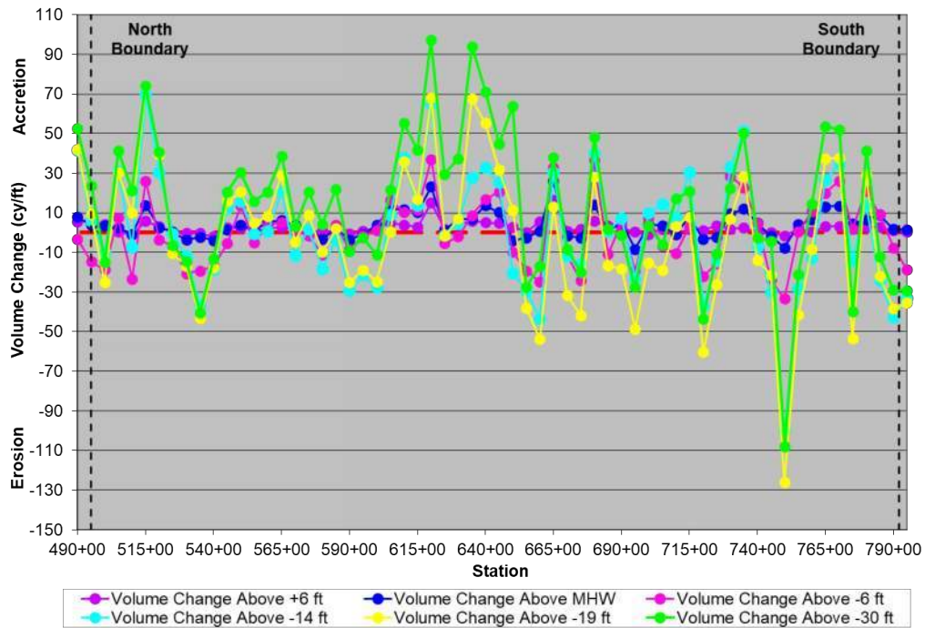
Figure 5-9. Nags Head – Reach 1 Unit Volume Change (June 2023 – June 2024)
