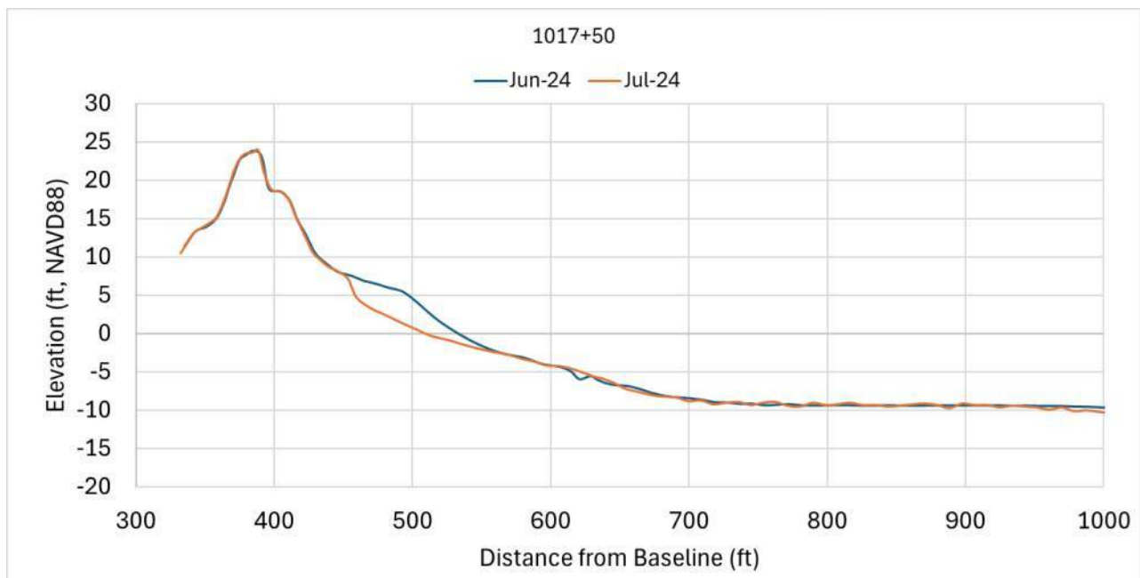
Figure 6. Transect STA 1017+50 Observed Change, June to July 2024.
