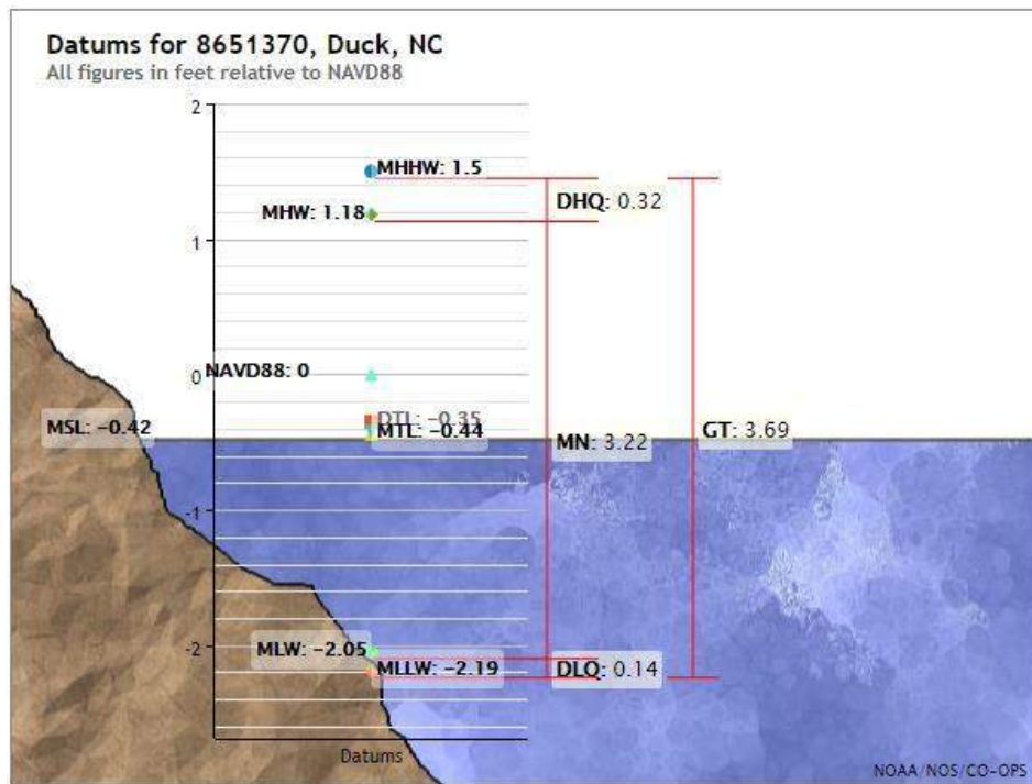
Figure 4-1. Tidal Datum for Duck, NC Station 8651370
