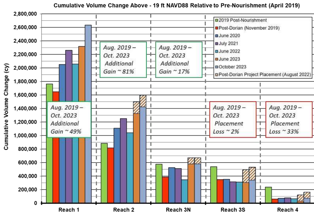
Figure 6-3. Cumulative Volume Change Above -19 ft NAVD88 Relative to Pre-Nourishment
