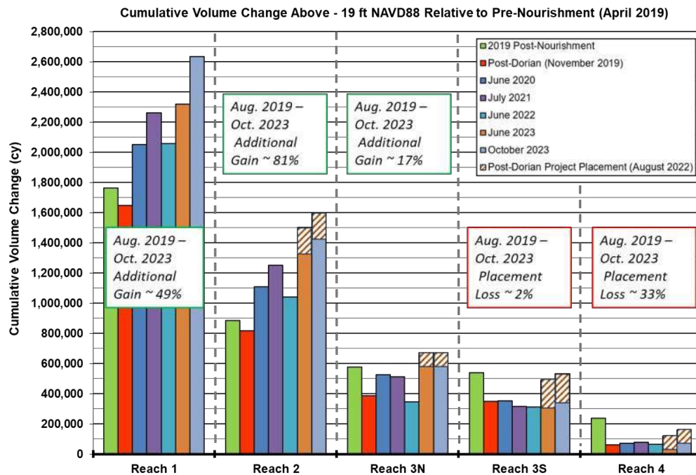
Figure ES-3. Cumulative Volume Change Above -19 ft NAVD88 Relative to Pre-Nourishment
