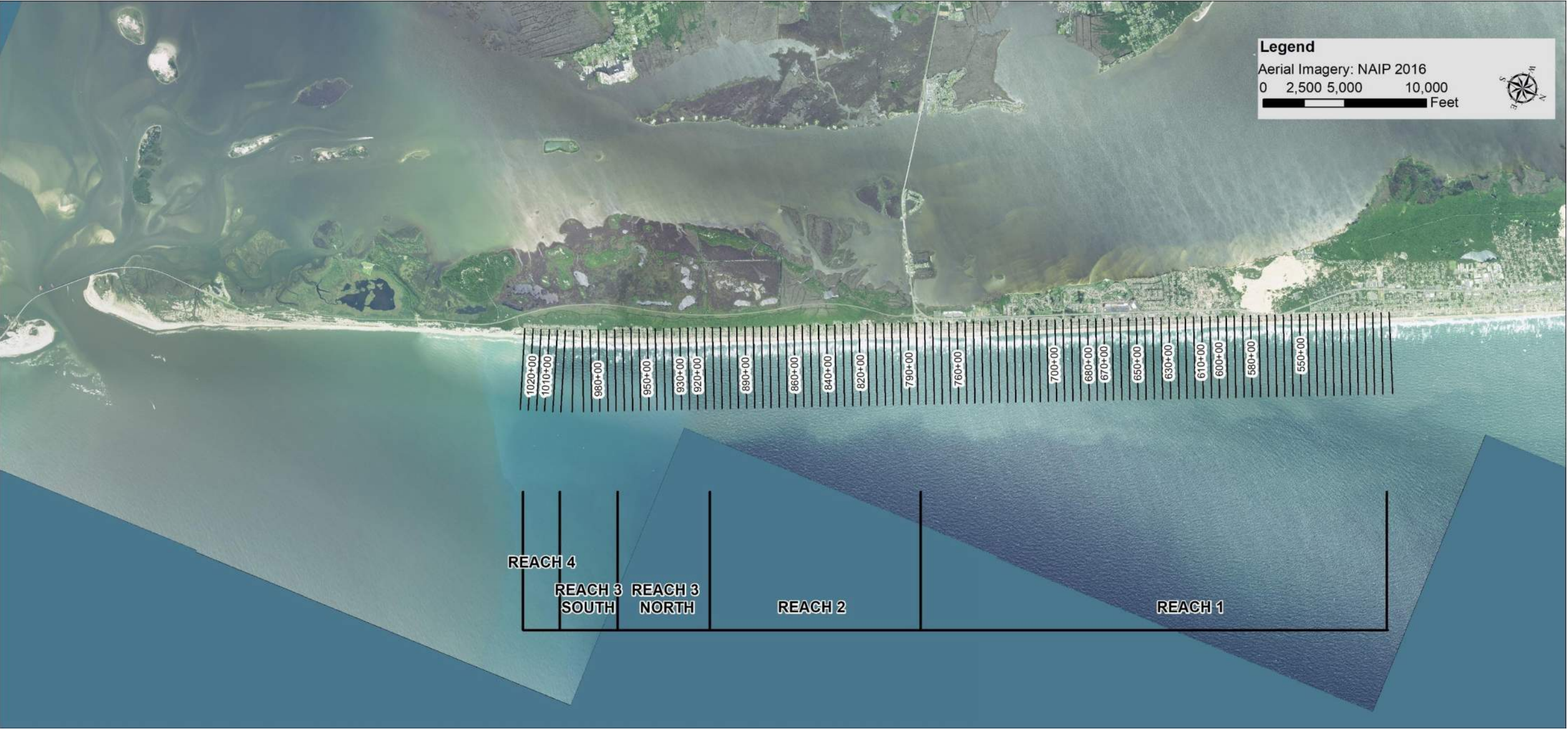
Figure 3-2. Nags Head Fall Monitoring Profile Line Locations
