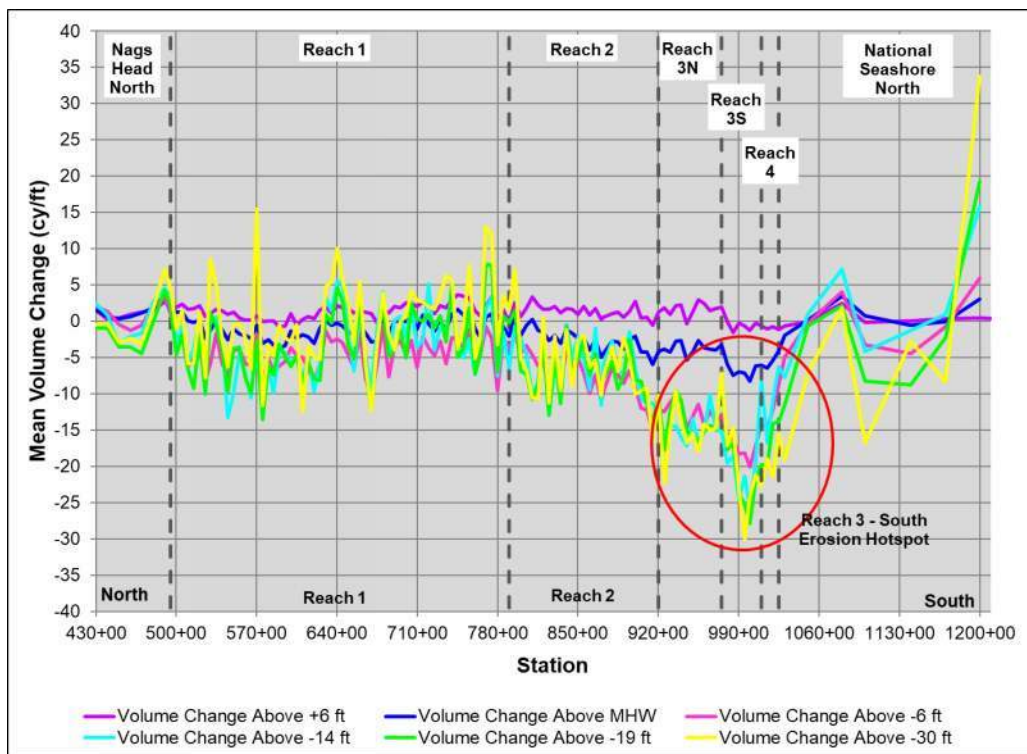
Figure 5-42. Mean Volume Change per year (2011 – 2024) (Without Nourishment)
