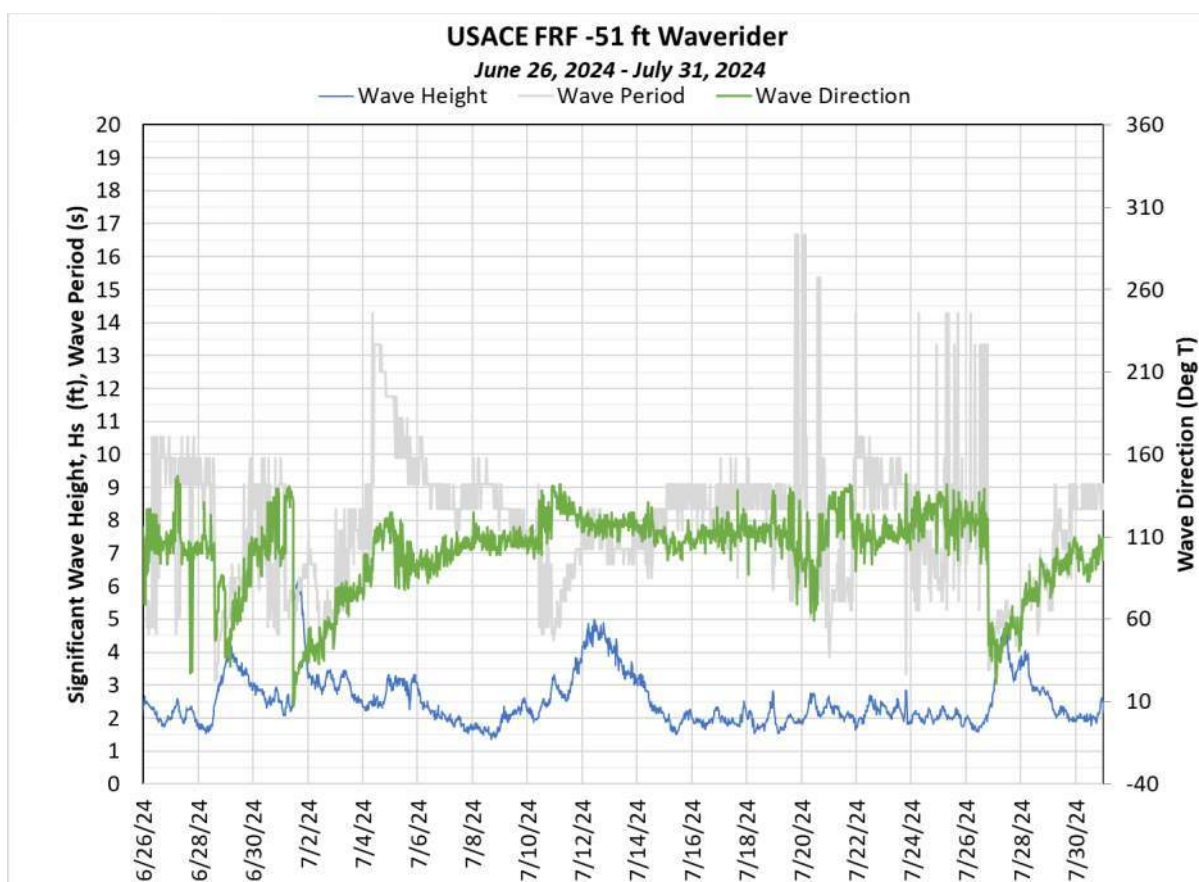
Figure 11. Wave Height (blue), Period (gray), and Direction (green) Time Series for June 26, 2024 to July 31, 2024, at Duck -51ft waverider buoy.
