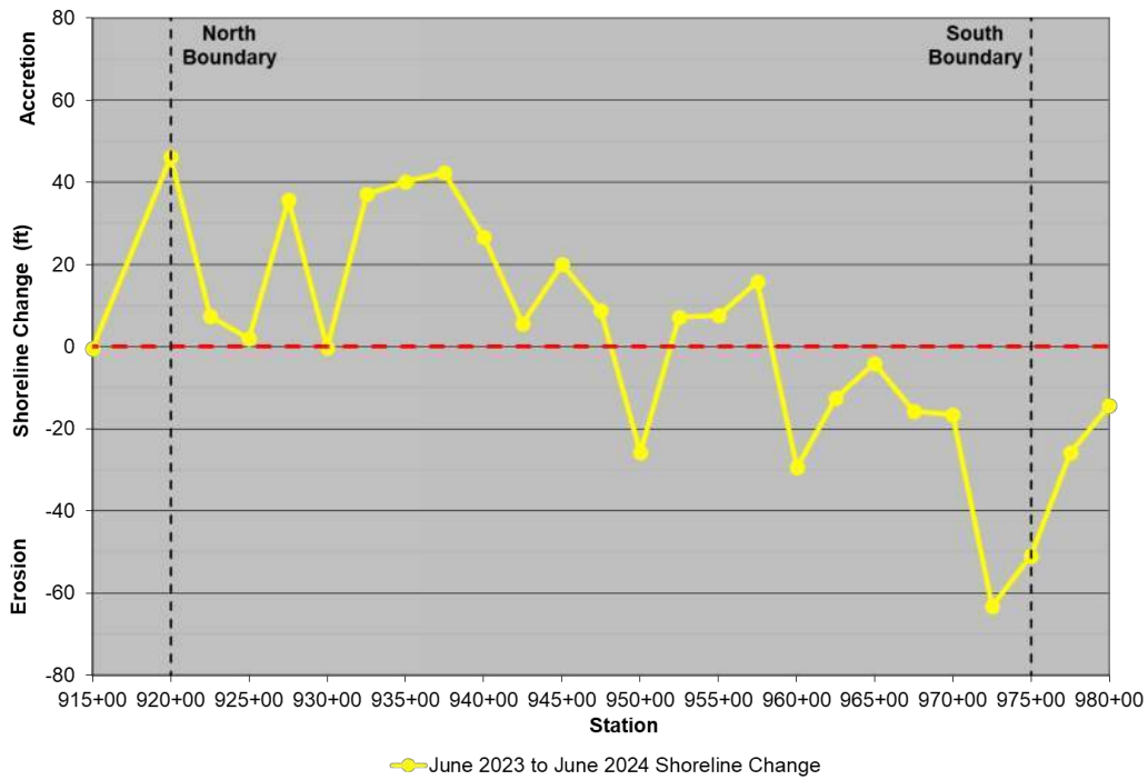
Figure 5-15. Nags Head – Reach 3 - N Shoreline Change (June 2023 – June 2024)
