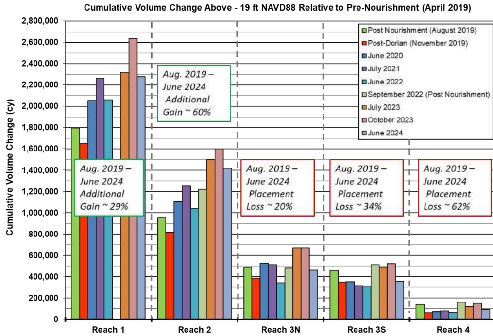
Figure 5-37. Cumulative Volume Change Above -19 ft NAVD88 Relative to Pre-Nourishment
