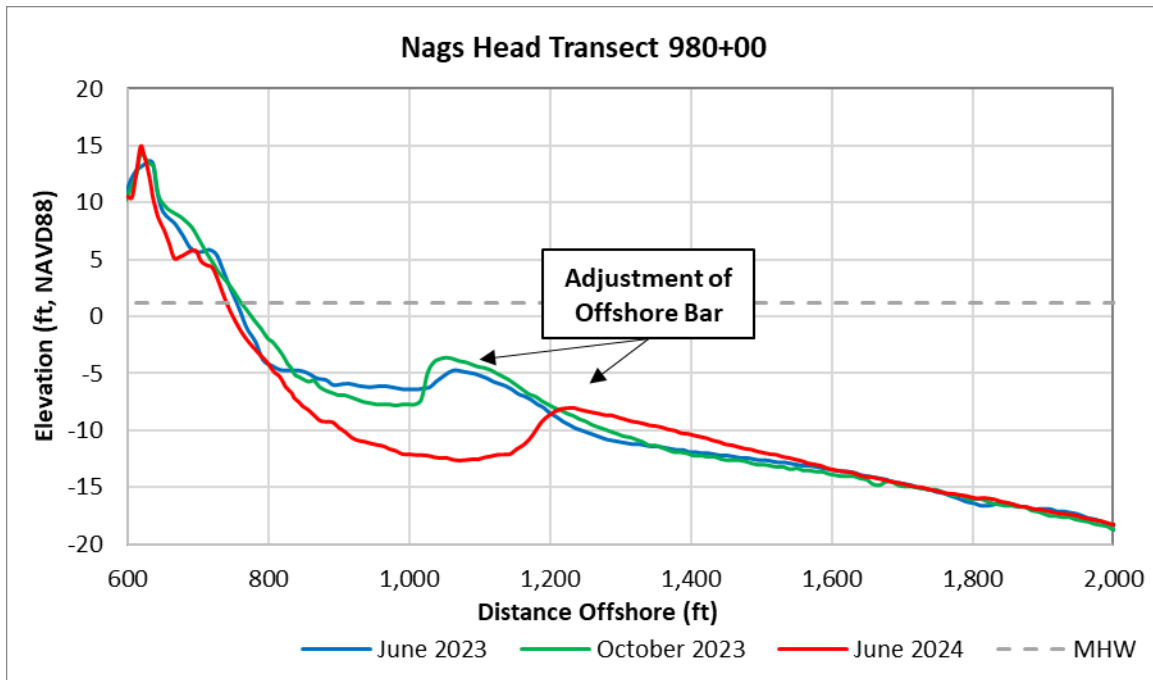
Figure 5-20. Example Reach 3 - South Profile, Station 980+00 (E Altoona St.)
