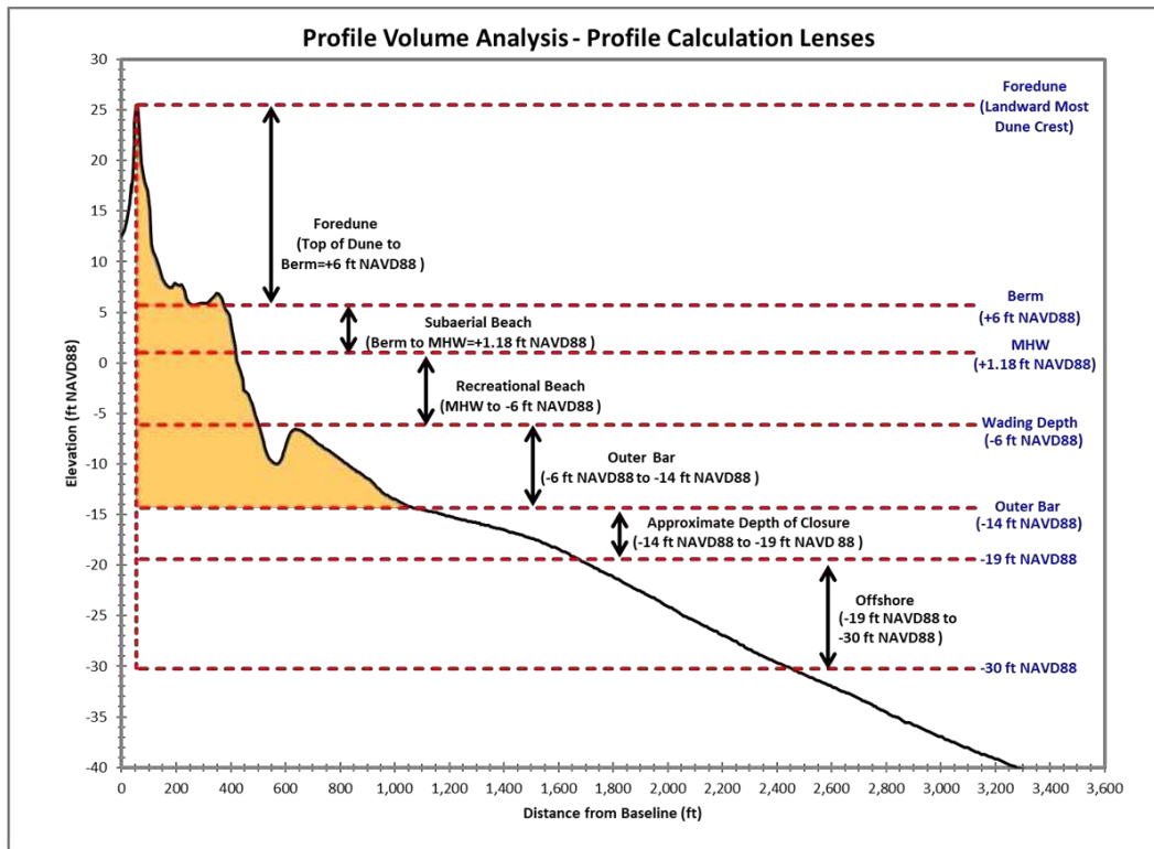
Figure 4-2. Profile Volume Calculation Lenses
